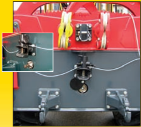
three-point-linkage with power take-off
